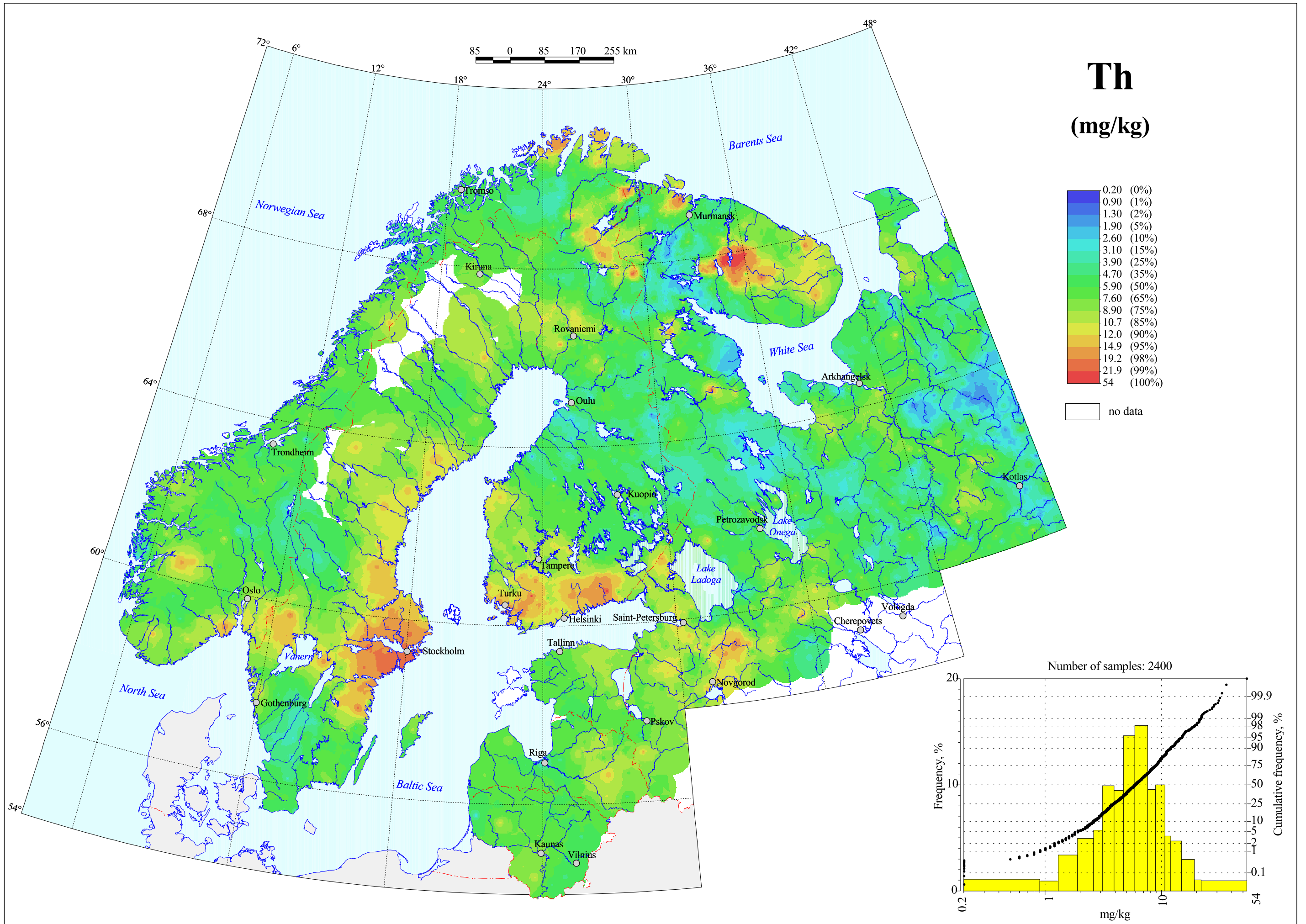
Thorium in C-horizon, Grain Size <math>< 2\text{ mm}</math>, Total Content
